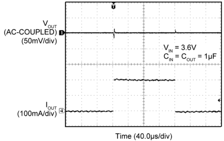
Load Transient (0mA to 200mA)
