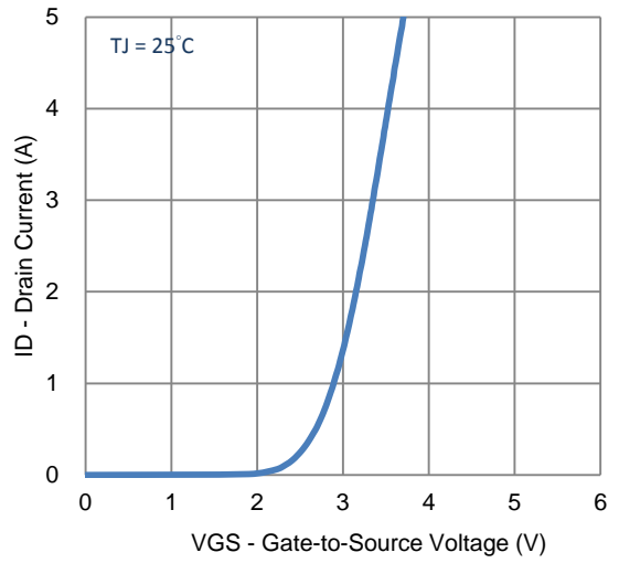
2. Transfer Characteristics
