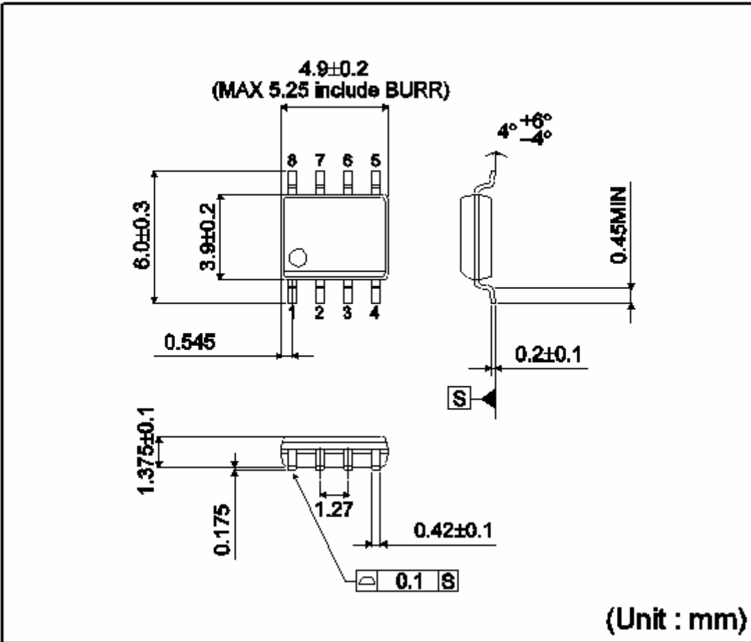
SOP-J8
