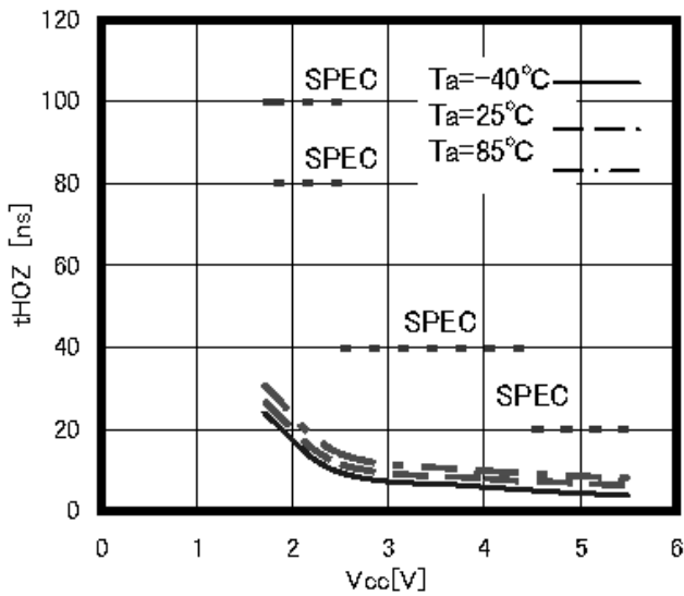
Figure 26. Time from HOLDB to output High-Z tHOZ
