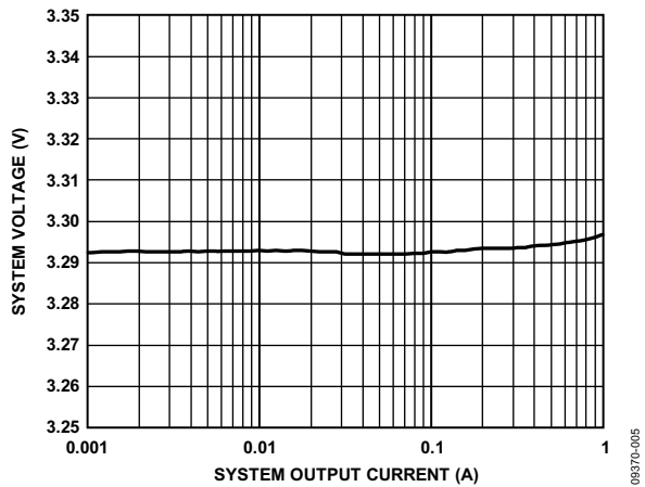
Figure 5. System Voltage Regulation vs. Output Current, V_{IN} = 5.0\text{ V}
