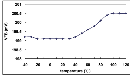
Figure 5. VFB vs. temperature
