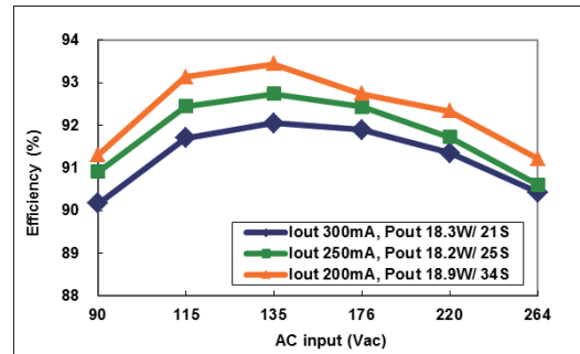
Figure 7. Efficiency vs. Wide AC Voltage
