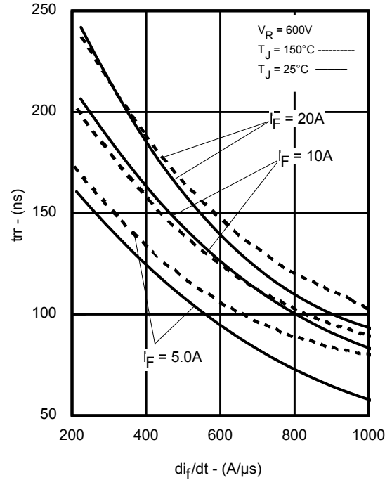
Fig 2. Typical t_{tr} vs. di/dt
