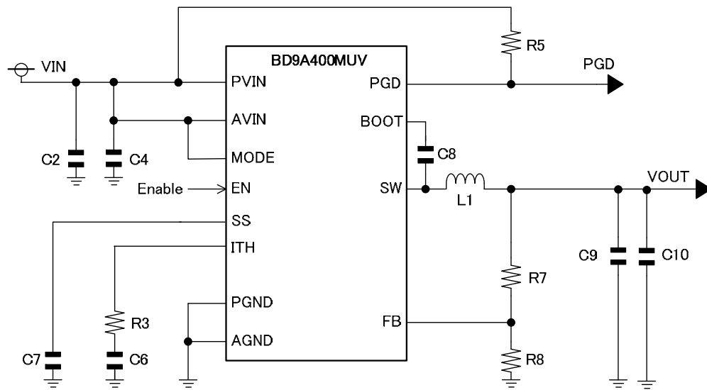
Figure 48. Application Circuit
