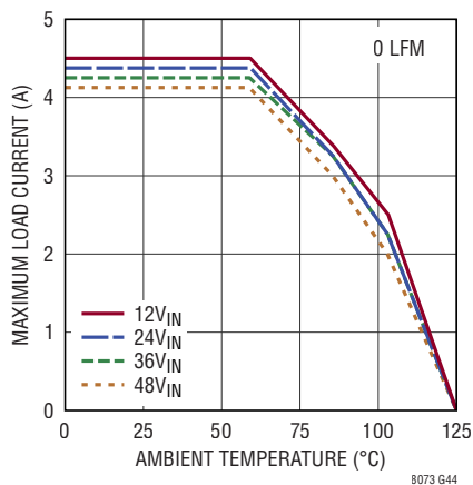
Derating, V_{OUT} = 2.5\text{V} , BIAS = 5V, DC2389A Demo Board
