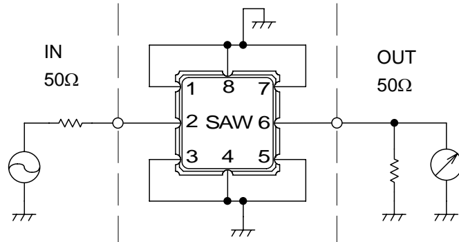
Fig.2 Measuring circuit
