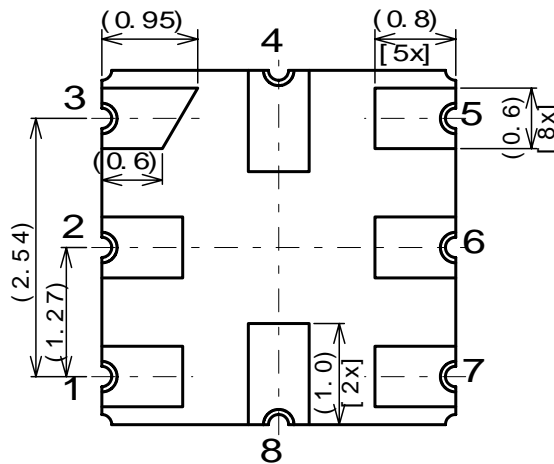
Fig.3 Package dimensions (in mm)
