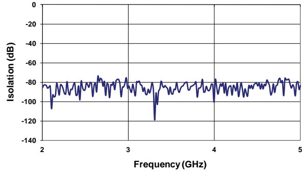
Isolation (2-5 GHz)
