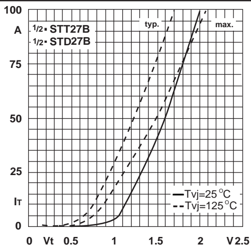
Fig.7 On-state characteristics
