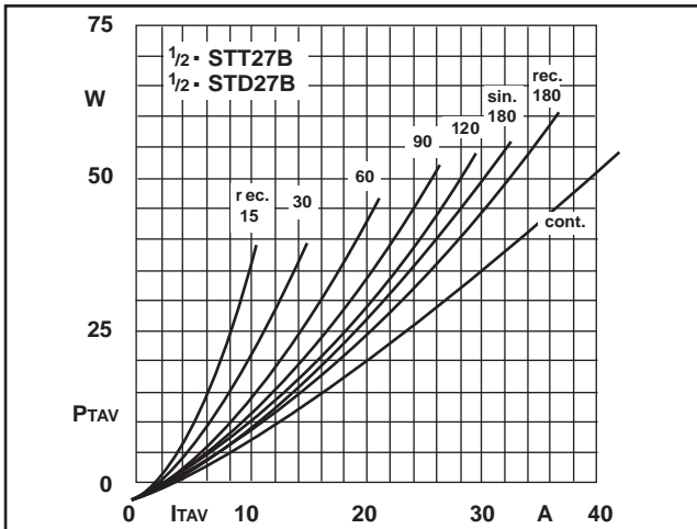
Fig.1L Power dissipation per thyristor vs. on-state current
