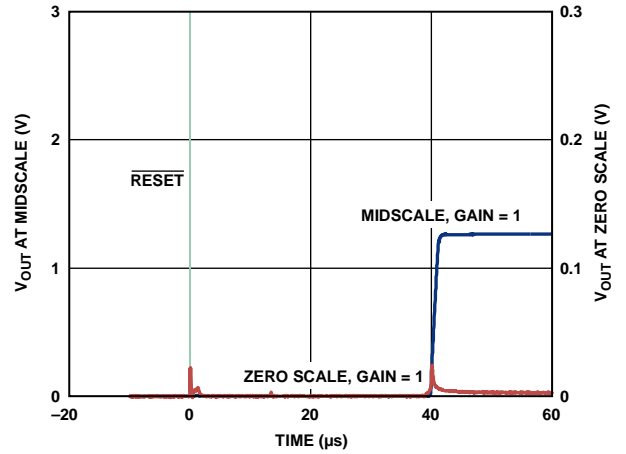
Figure 38. Hardware Reset
