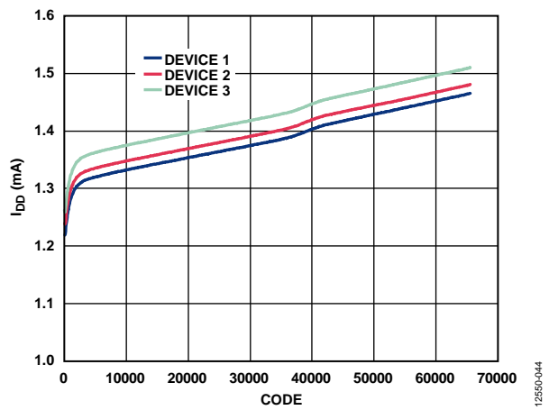
Figure 23. Supply Current ( I_{DD} ) vs. Code
