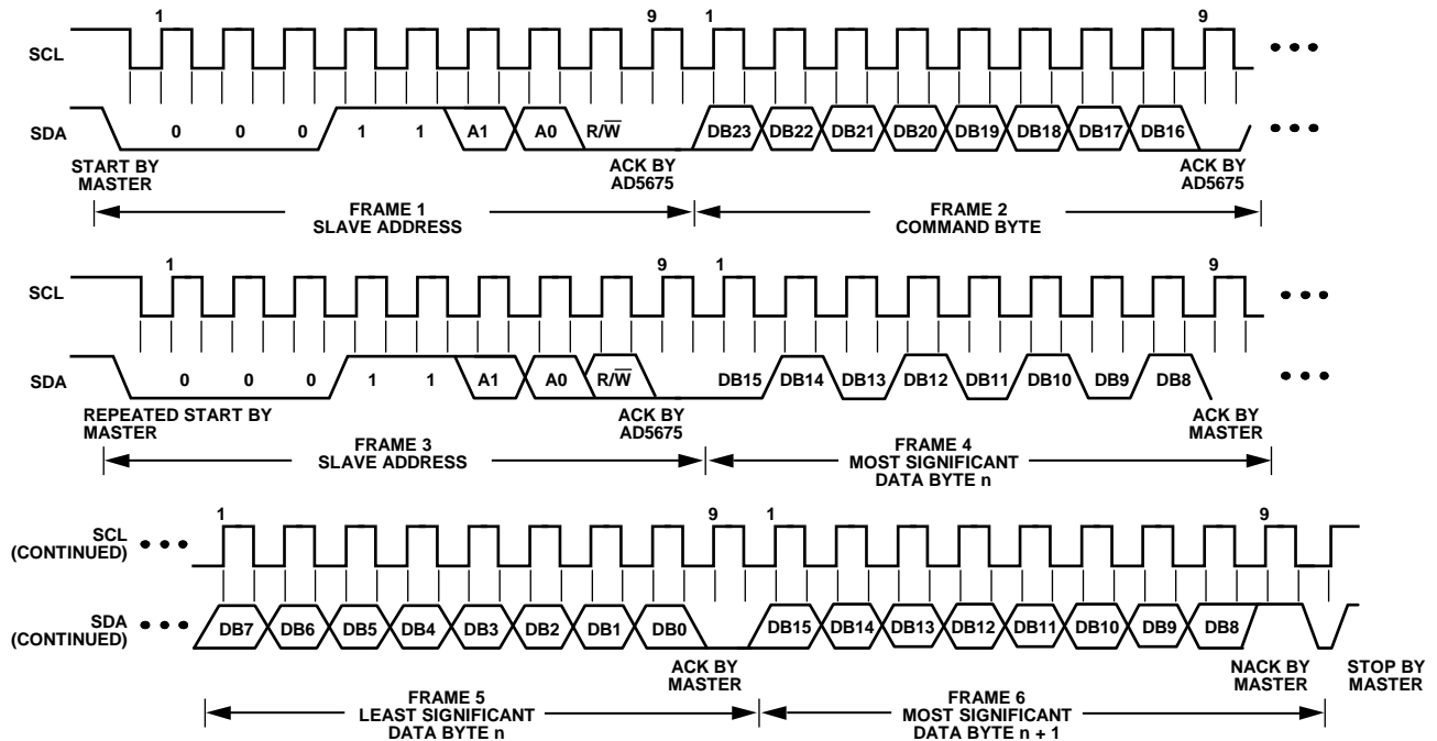
Figure 44. PC Read Operation
