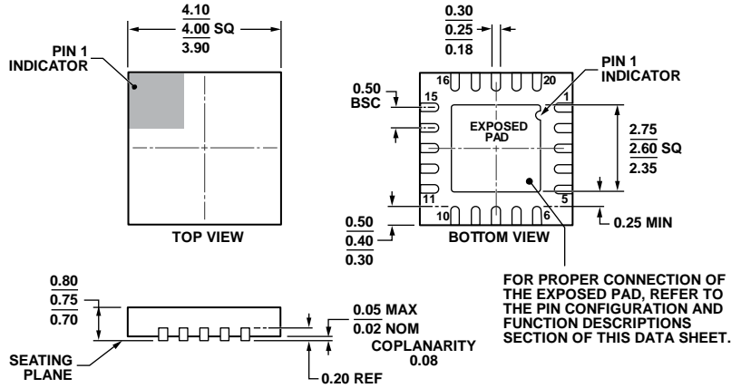
Figure 52. 20-Lead Lead Frame Chip Scale Package [LFCSP] 4 mm x 4 mm Body and 0.75 mm Package Height
