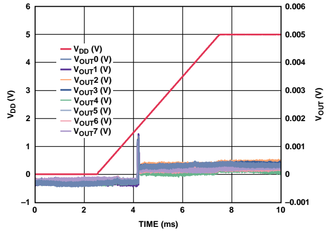
Figure 28. Power-On Reset to 0 V and Midscale
