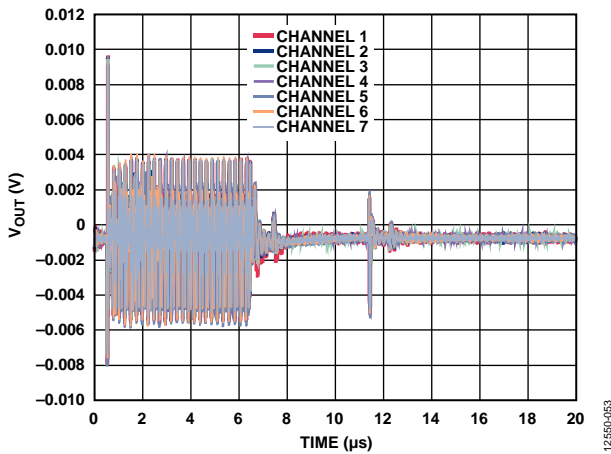
Figure 32. DAC-to-DAC Crosstalk
