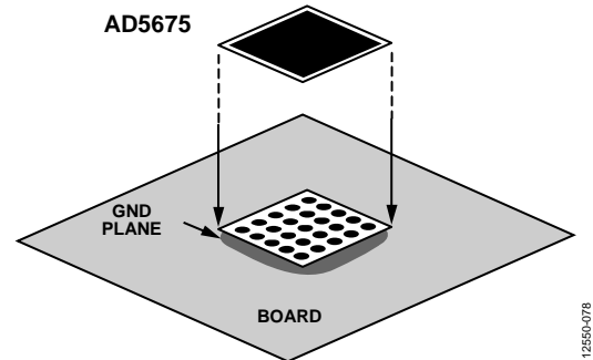
Figure 49. Pad Connection to Board
