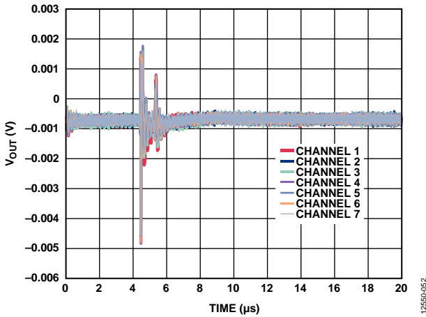
Figure 31. Analog Crosstalk
