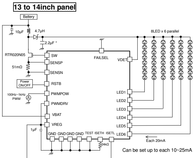
Figure 49. 8 series x parallel, LED current 20mA setting Power control PWM application;:n
