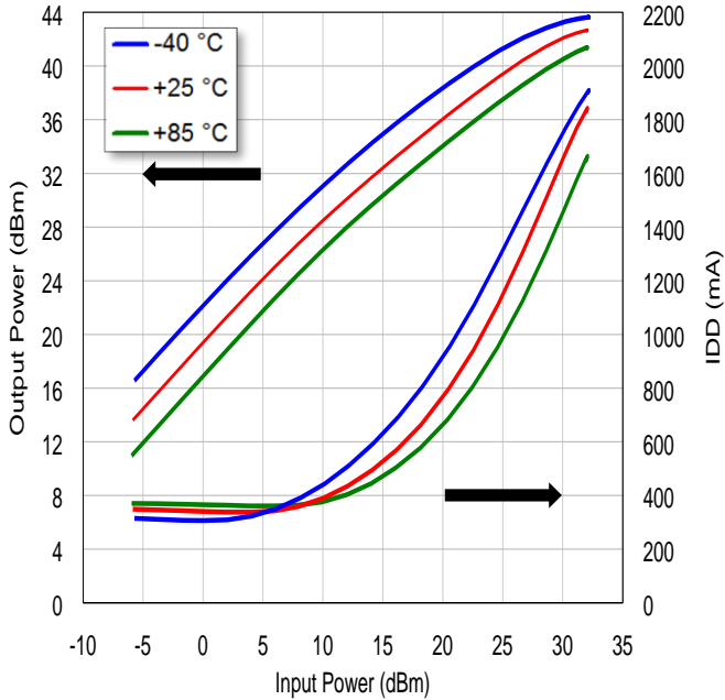
VDD = +28 V, IDD = 350 mA @ 13.75 GHz
