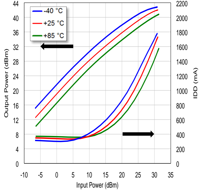
VDD = +28 V, IDD = 350 mA @ 14.00 GHz
