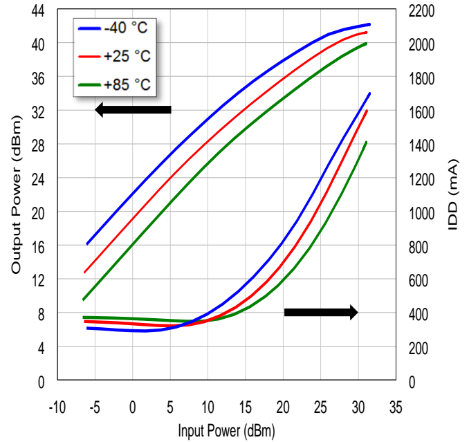
VDD = +28 V, IDD = 350 mA @ 14.50 GHz
