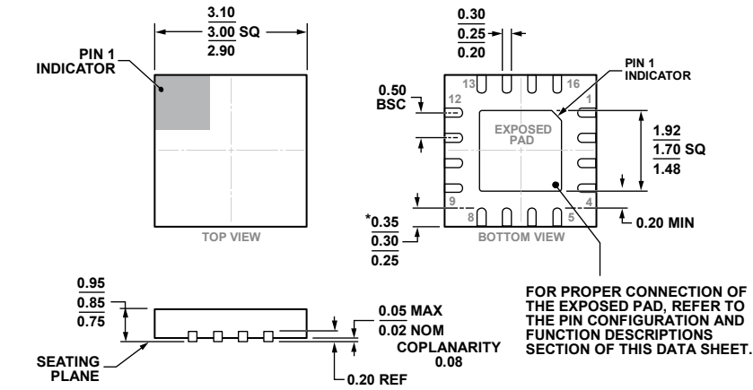
*COMPLIANT WITH JEDEC STANDARDS MO-220-VEED-4 WITH THE EXCEPTION OF PACKAGE EDGE TO LEAD EDGE. Figure 20. 16-Lead Lead Frame Chip Scale Package [LFCSP_WQ] 3 mm x 3 mm Body, Very Very Thin Quad (CP-16-38) Dimensions shown in millimeters
