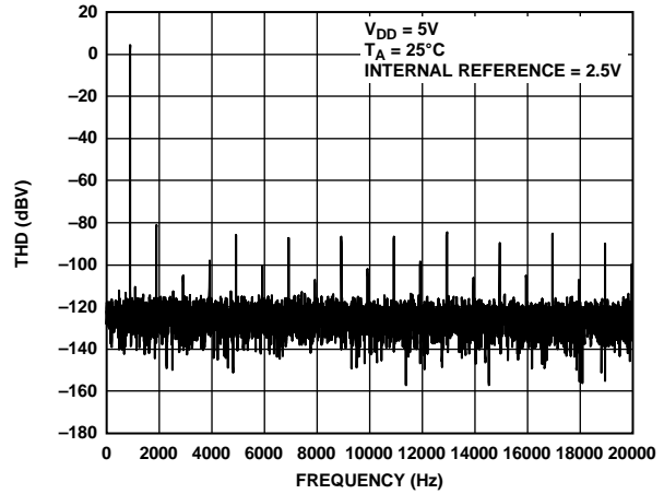
Figure 38. Total Harmonic Distortion at 1 kHz
