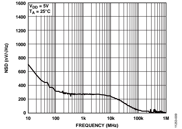
Figure 8. Internal Reference Noise Spectral Density vs. Frequency
