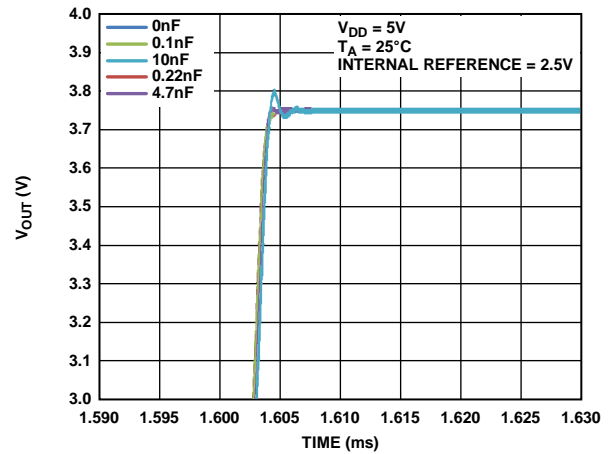
Figure 39. Settling Time vs. Capacitive Load
