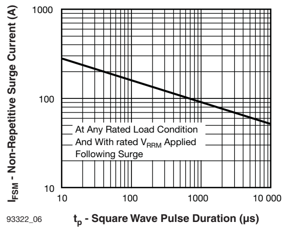
93322_06 t p - Square Wave Pulse Duration (μs) Fig. 6 - Maximum Non-Repetitive Surge Current
