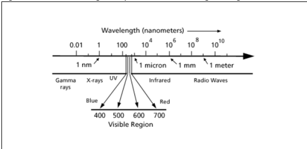
Figure 2. The electromagnetic spectrum and visible region of light
