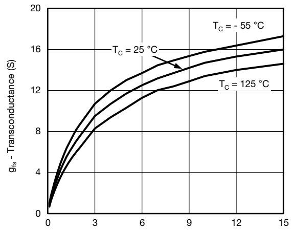
Transconductance
