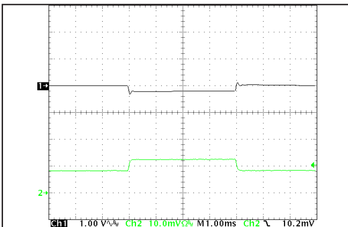
Figure 11: Output voltage response to step-change in load current (50%-75%-50% of I_{out(max)} ; dI/dt = 0.1 A/\mu s ). Load cap: 15 \mu F tantalum cap and 1 \mu F ceramic cap. Ch 1: V_{out} (1 V/div), Ch 2: I_{out} (50 A/div).
