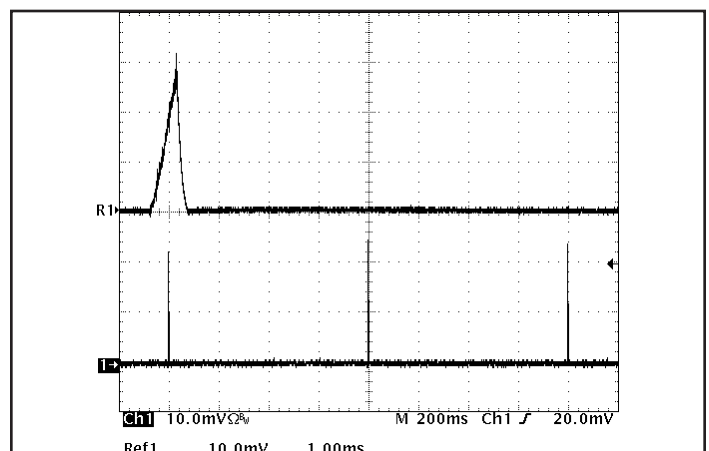
Figure 18: Load current (50 A/div) as a function of time when the converter attempts to turn on into a 1 \text{m}\Omega short circuit. Top trace (1 ms/div) is an expansion of the on-time portion of the bottom trace.
