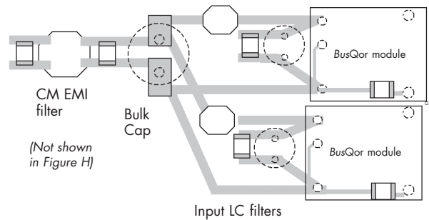
Figure H: Recommended PCB layout for input circuit
