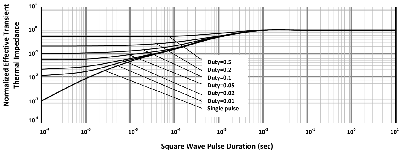
Normalized Thermal Transient Impedance, Junction-to-Case (DPAK/IPAK)
