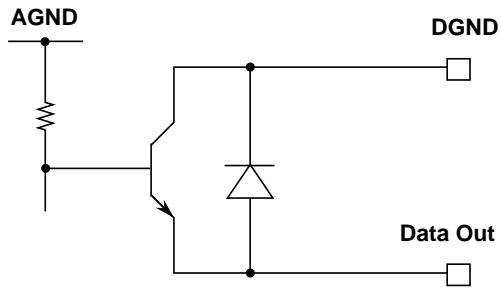
Figure 3 - Output Circuit
