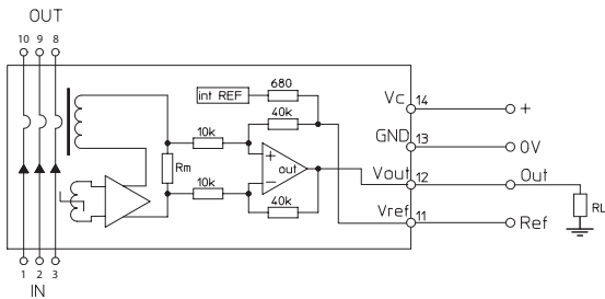
Figure 31: Test connection
