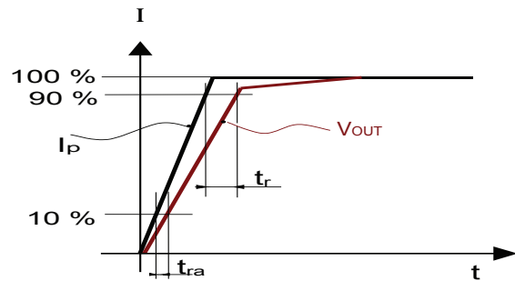
Figure 32: Response time t_r and reaction time t_{ra}
