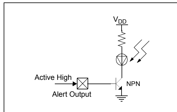
FIGURE 6-3: Alert Output Buffer.
