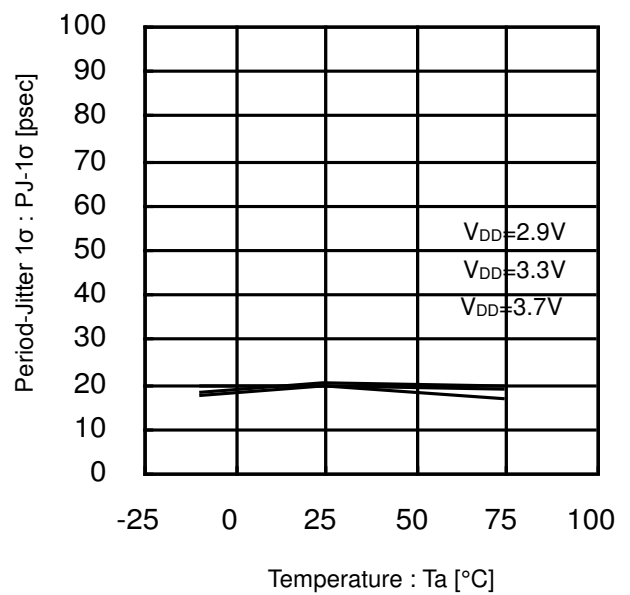
Figure 29. Period-Jitter 1σ vs Temperature (108MHz)
