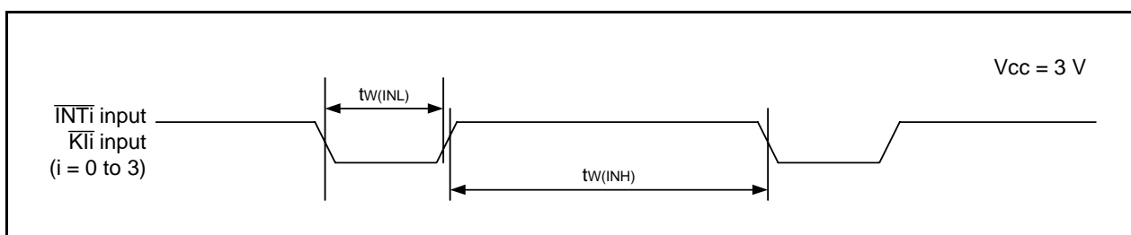
Figure 4.15 Timing for External Interrupt \overline{INTi} Input and Key Input Interrupt \overline{Kli} When Vcc = 3 V
