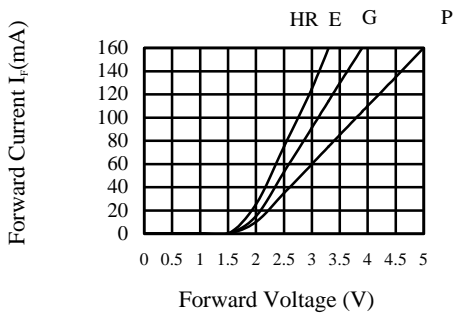
FIG.4 FORWARD CURRENT VS. FORWARD VOLTAGE
