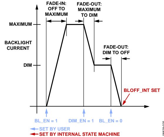
Figure 48. End of Fade-Out (EOF) Interrupt as Used for a Backlight Fade-Out (Set by User)
