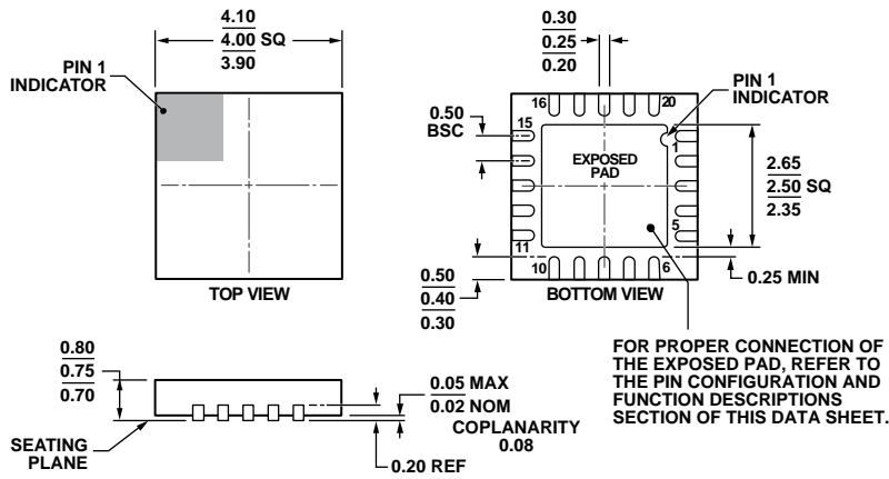
COMPLIANT TO JEDEC STANDARDS MO-220-WGGD. Figure 55. 20-Lead Lead Frame Chip Scale Package [LFCSP_WQ] 4 mm × 4 mm Body, Very Very Thin Quad (CP-20-10) Dimensions shown in millimeters
