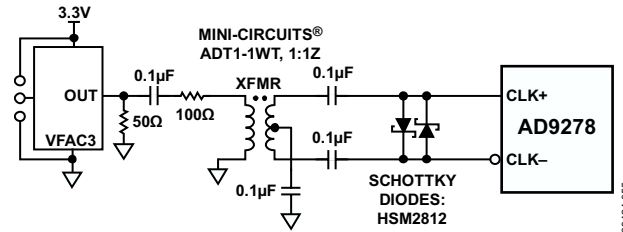
Figure 50. Transformer-Coupled Differential Clock
