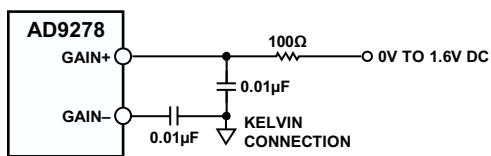
Figure 48. Single-Ended \text{GAIN}\pm Pin Configuration
