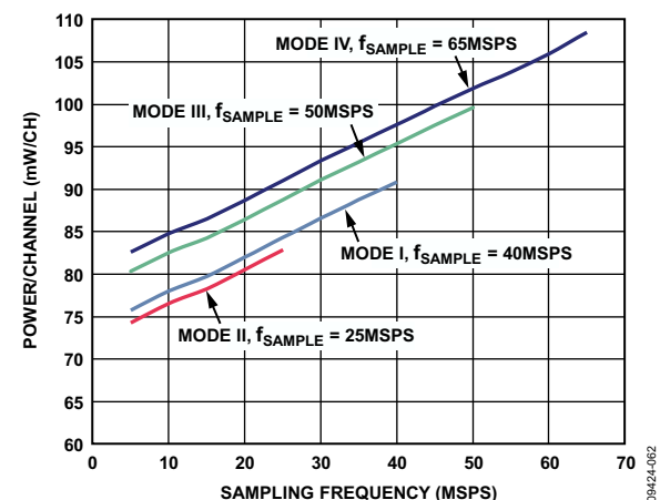
Figure 57. Power per Channel vs. f_{SAMPLE} for f_{IN} = 5 MHz
