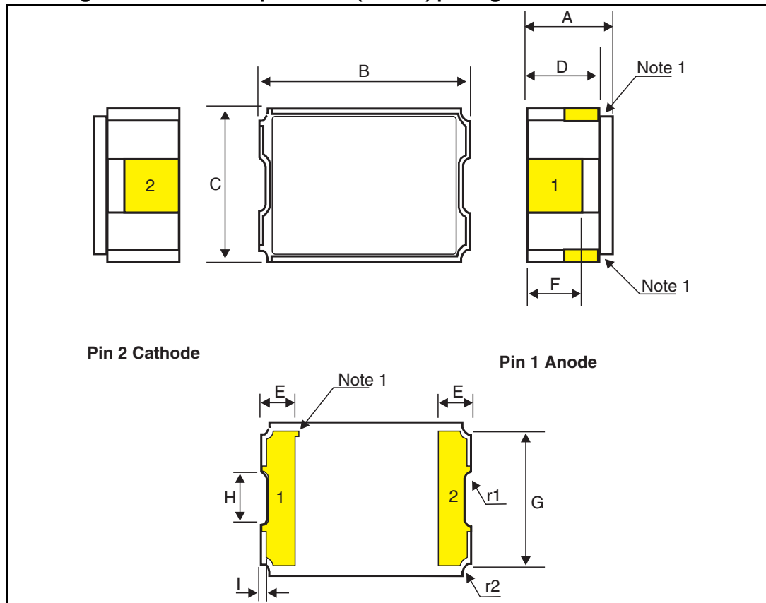
Figure 8. Leadless chip carrier 2 (LCC2B) package dimension definitions
