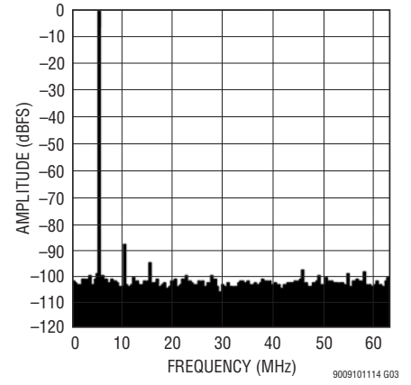
LTM9011-14: 8k Point FFT, f_{IN} = 5\text{MHz} , -1dBFS, 125Mpsps
