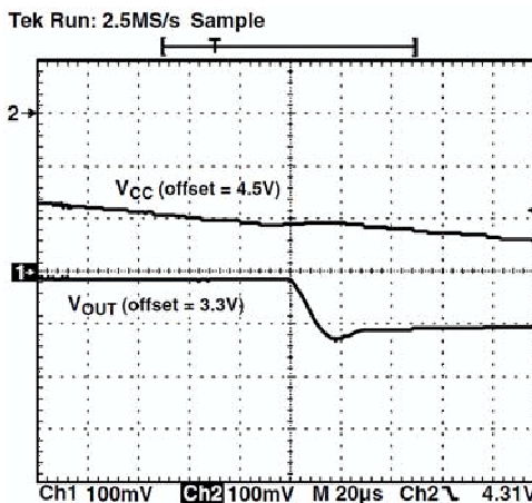
Figure 20. V_{CC} Power Down ( V_{AUX} = 3.3\text{ V} , Load = 300 mA)
