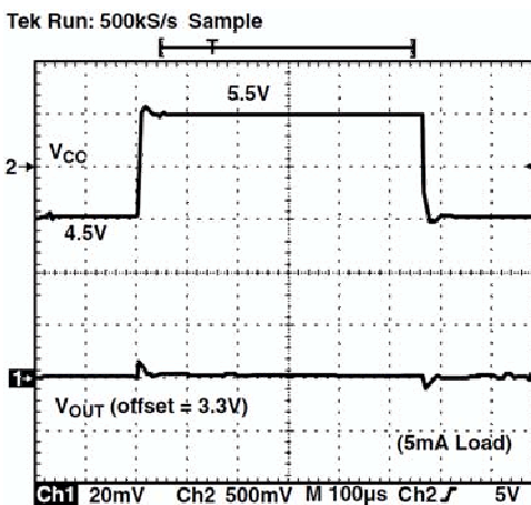
Figure 22. Line Transient (1 V_{PP} ) Response
