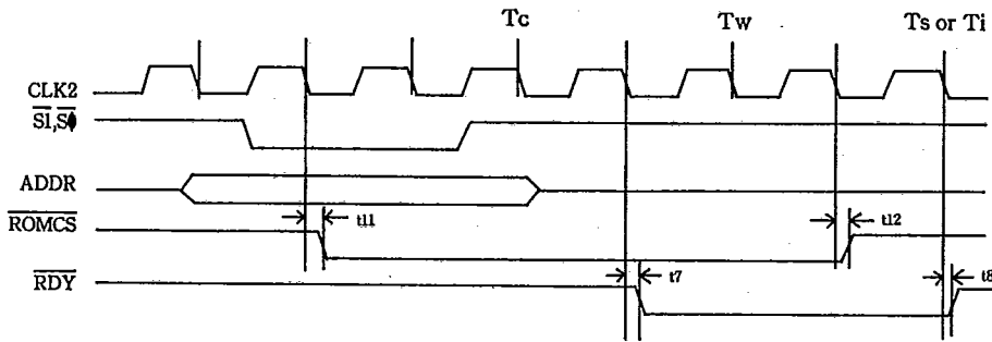
ROM Cycle
