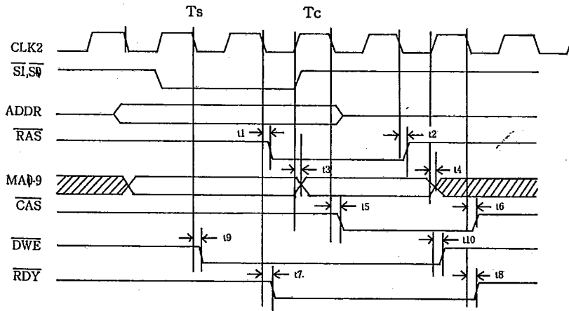
0 W.S. Write
