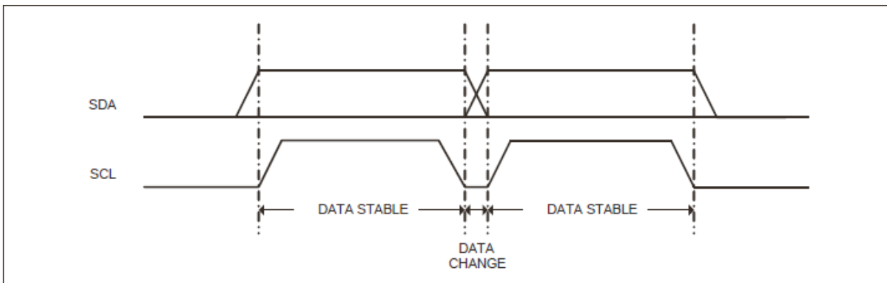
Figure 1: Data Validity
