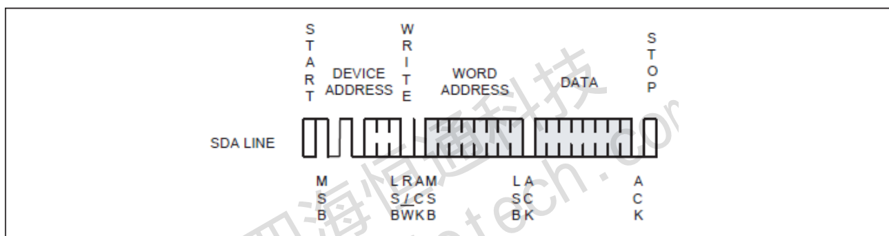
Figure 5: Byte Write
