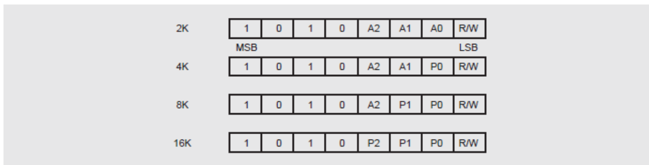
Figure 4: Device Address
