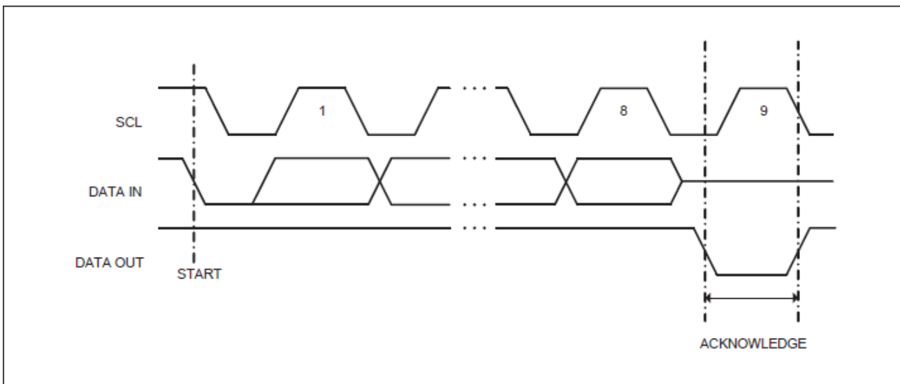
Figure 3: Output Acknowledge
