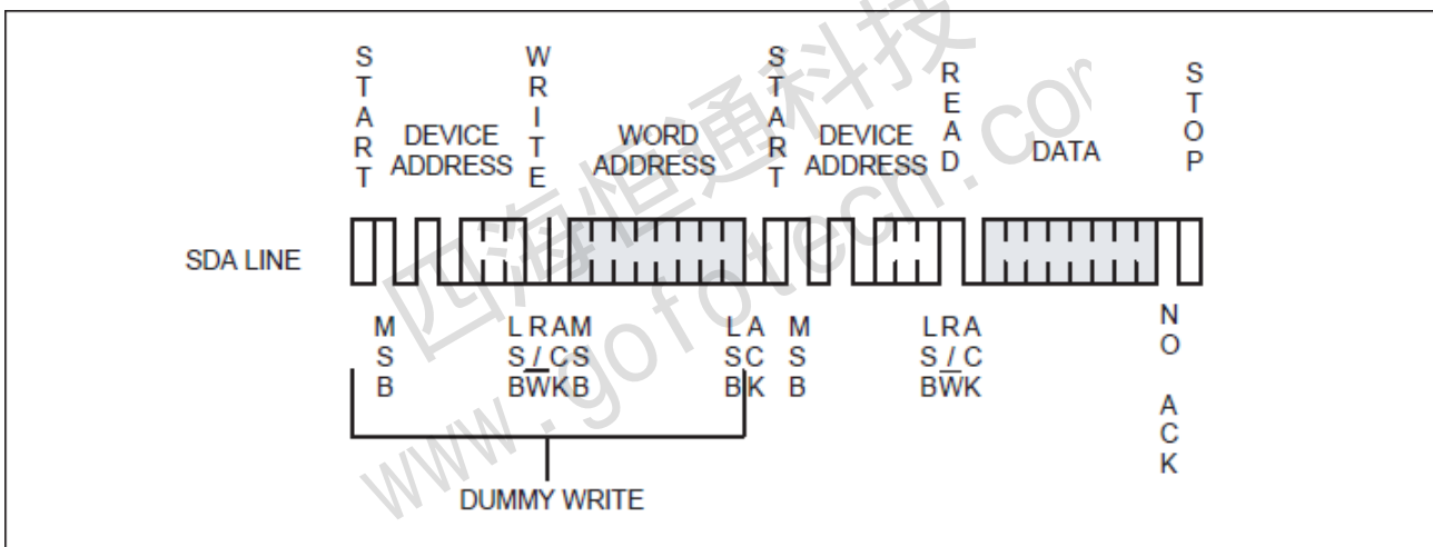
Figure 8: Random Read
