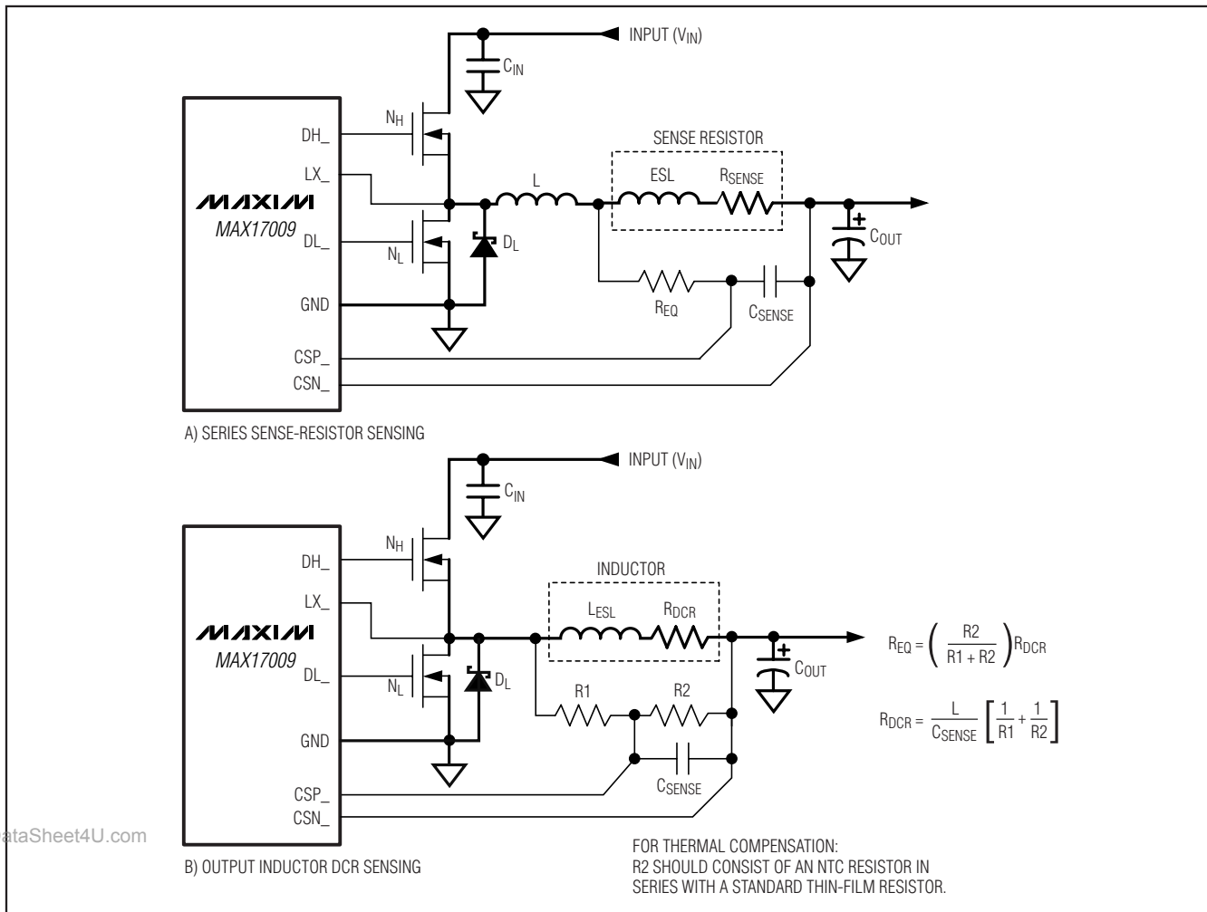
Figure 5. Current-Sense Configurations
