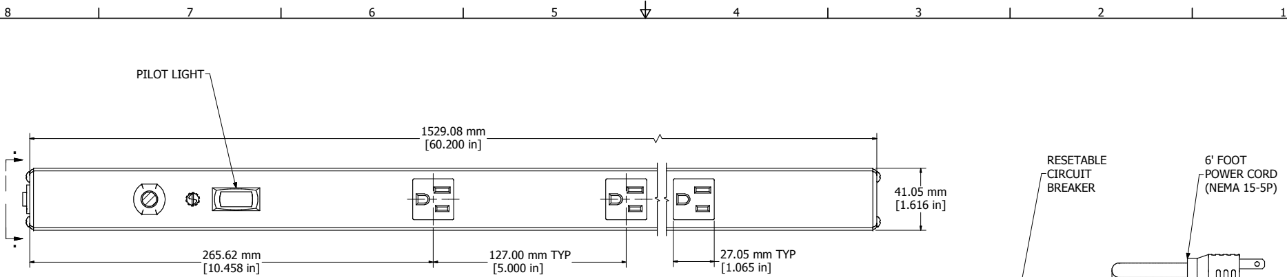
SECTION A-A (VIEW FROM FRONT)
