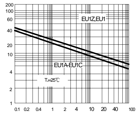
FIG.3–TYPICAL JUNCTION CAPACITANCE
