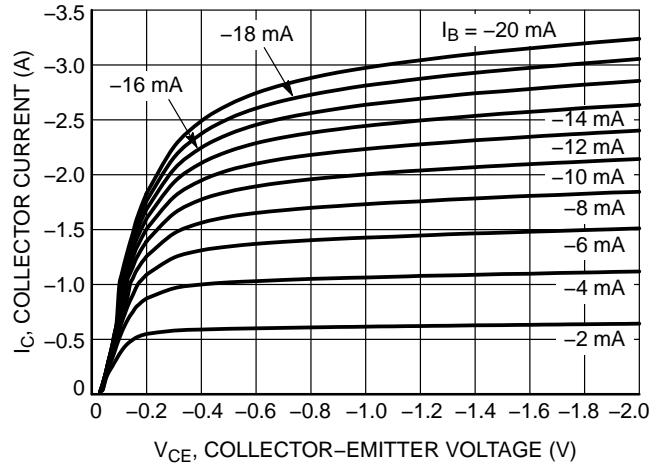
Figure 20. Output Characteristics
