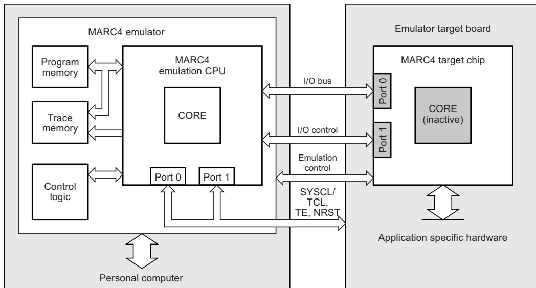
Figure 7-19. MARC4 Emulation
