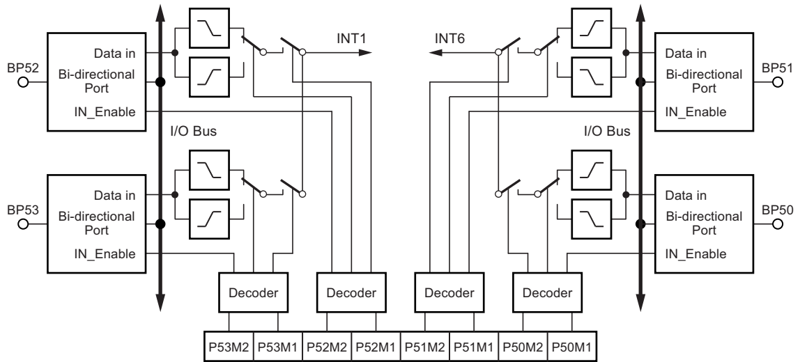
Figure 4-4. Port 5 External Interrupts
