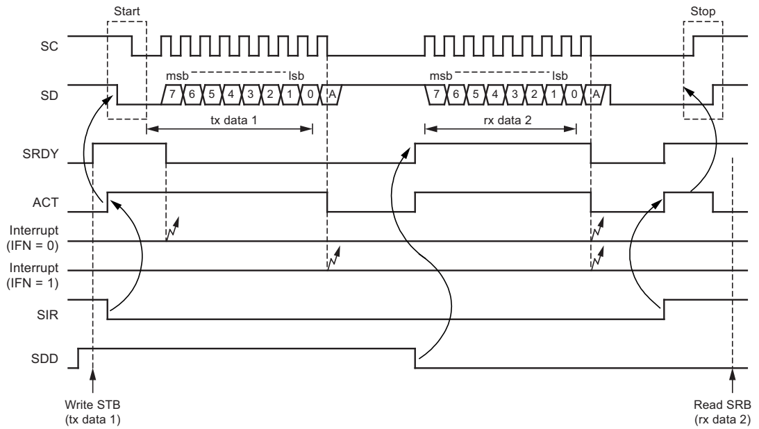
Figure 4-28. Example of MCL Receive Dialog
