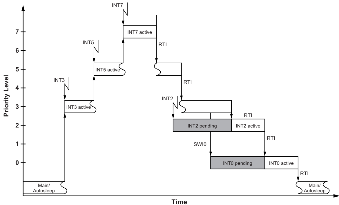
Figure 3-6. Interrupt Handling
