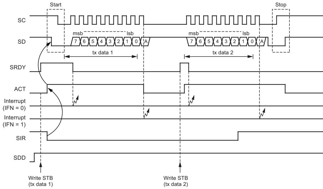
Figure 4-27. Example of MCL Transmit Dialog
