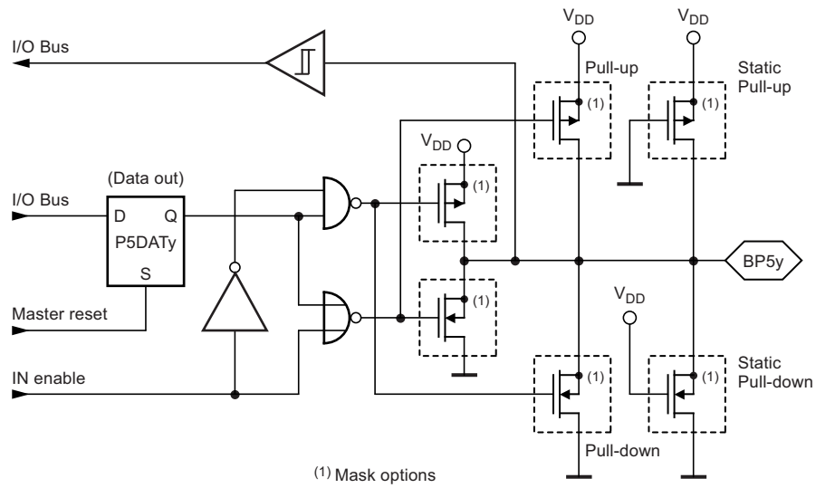
Figure 4-3. Bi-directional Port 5
