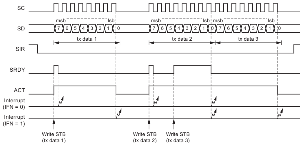
Figure 4-25. Example of 8-bit Synchronous Transmit Operation
