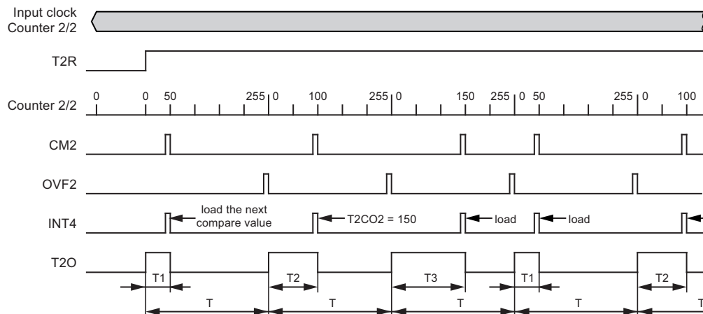
Figure 4-21. PWM Modulation
