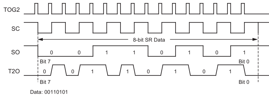
Figure 4-35. Manchester Modulation 1
