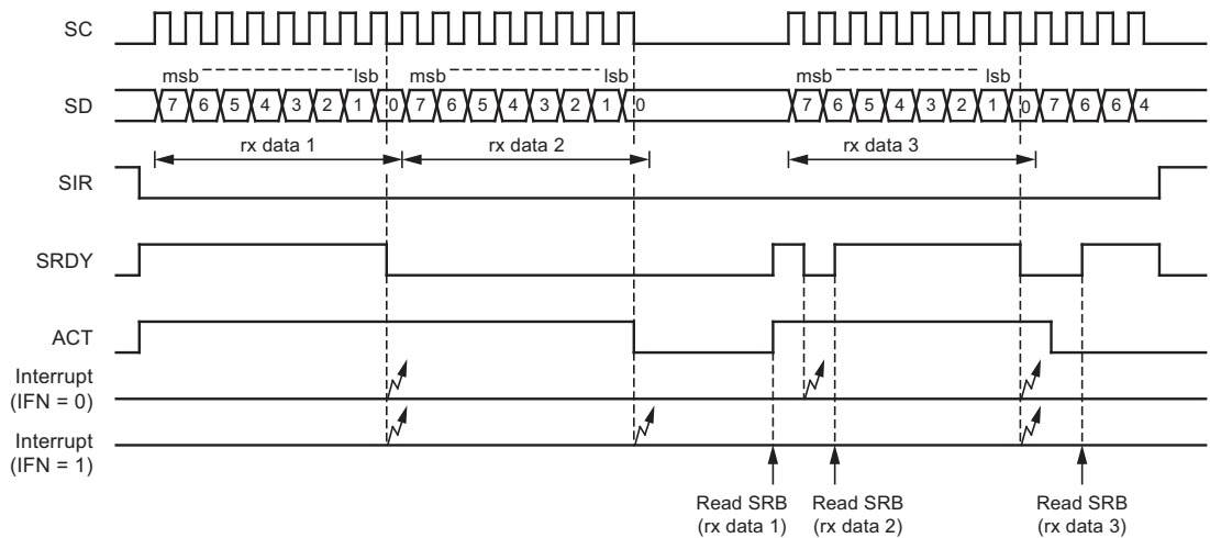
Figure 4-26. Example of 8-bit Synchronous Receive Operation
