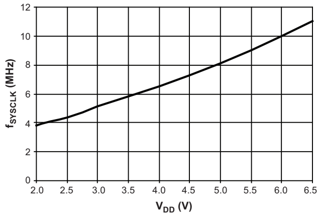
Figure 7-7. Maximum System Clock versus V_{DD}
