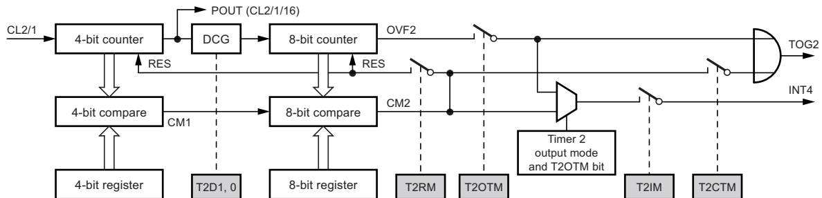
Figure 4-10. 12-bit Compare Counter
