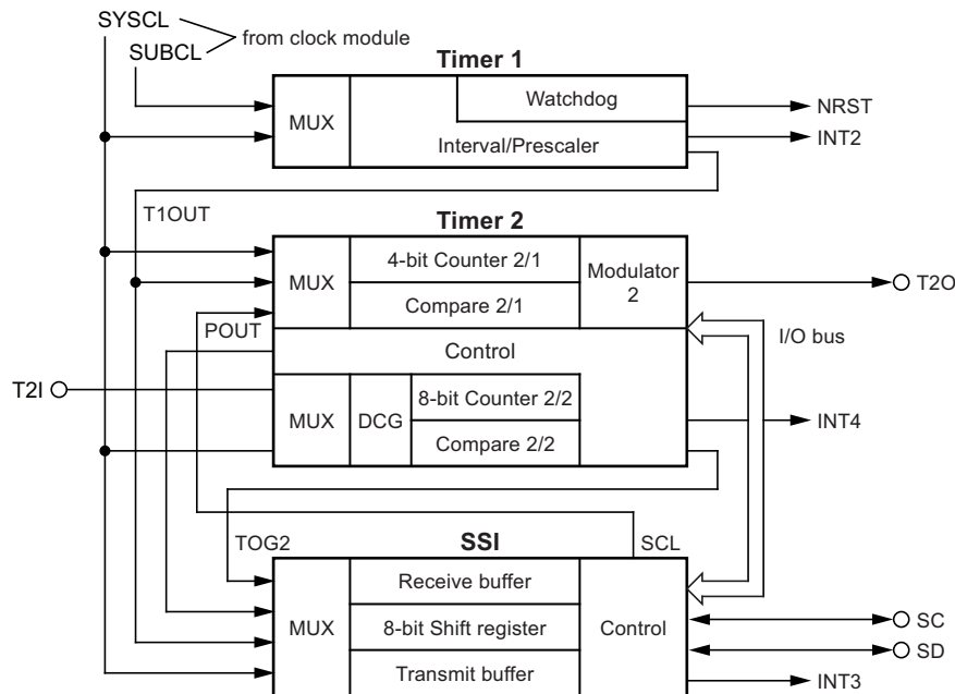
Figure 4-6. UTCM Block Diagram
