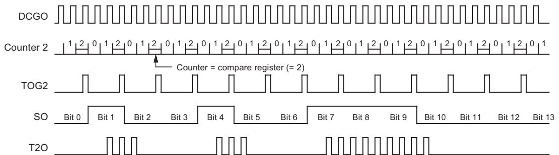
Figure 4-18. Carrier Frequency Burst Modulation with SSI Data Output
