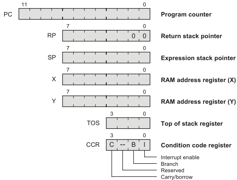
Figure 3-4. Programming Model
