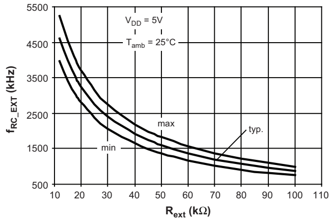
Figure 7-10. External RC Frequency versus R_{ext}
