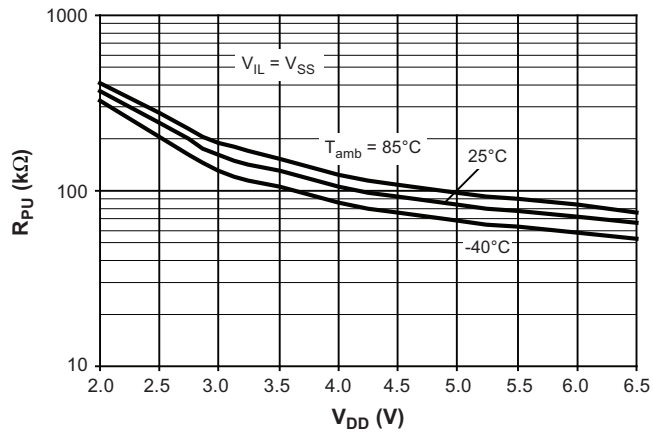
Figure 7-12. Strong Pull-up Resistor versus V_{DD}
