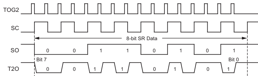
Figure 4-19. Bi-phase Modulation
