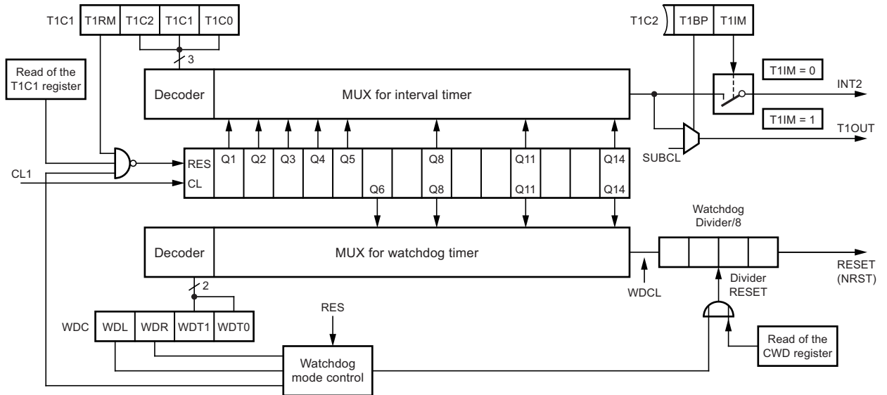
Figure 4-8. Timer 1 and Watchdog
