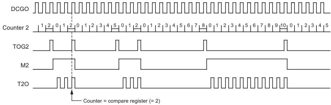
Figure 4-17. Carrier Frequency Burst Modulation with Timer 2 Toggle Flip-Flop Output
