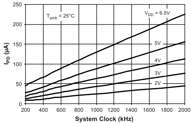
Figure 7-2. Power-down Supply Current versus Frequency
