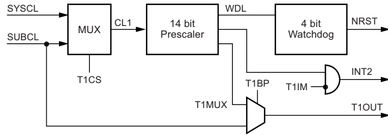
Figure 4-8. Timer 1 and Watchdog
