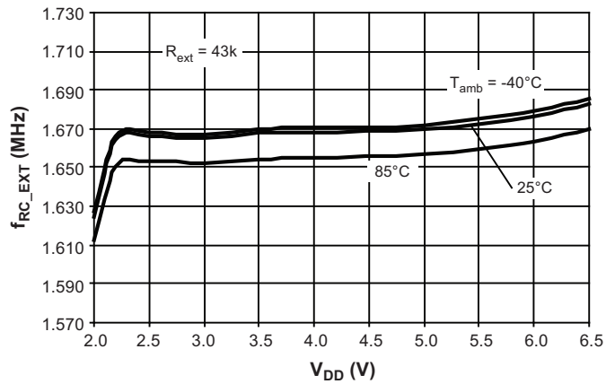
Figure 7-6. External RC Frequency versus V_{DD}
