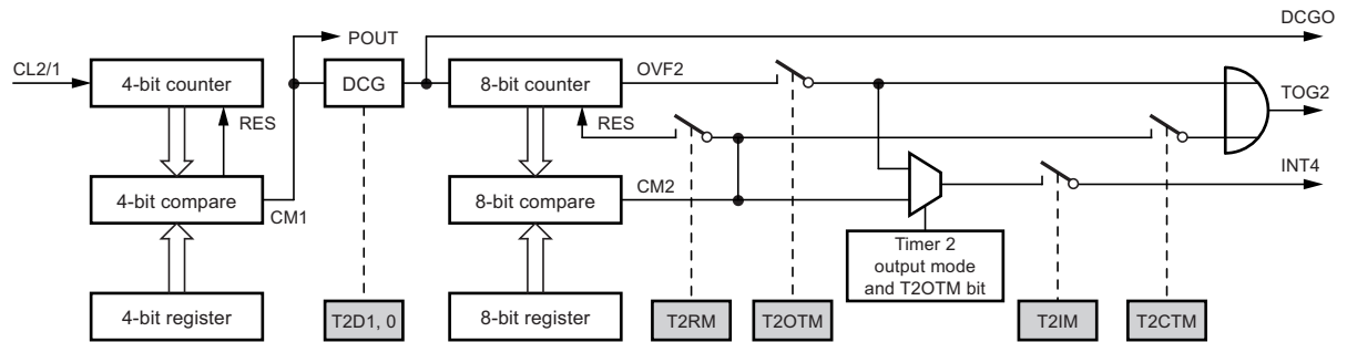
Figure 4-11. 8-bit Compare Counter
