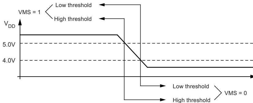
Figure 3-10. Internal Supply Voltage Supervisor
