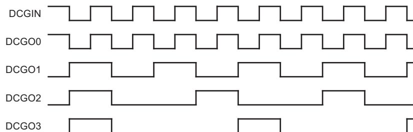
Figure 4-22. DCG Output Signals
