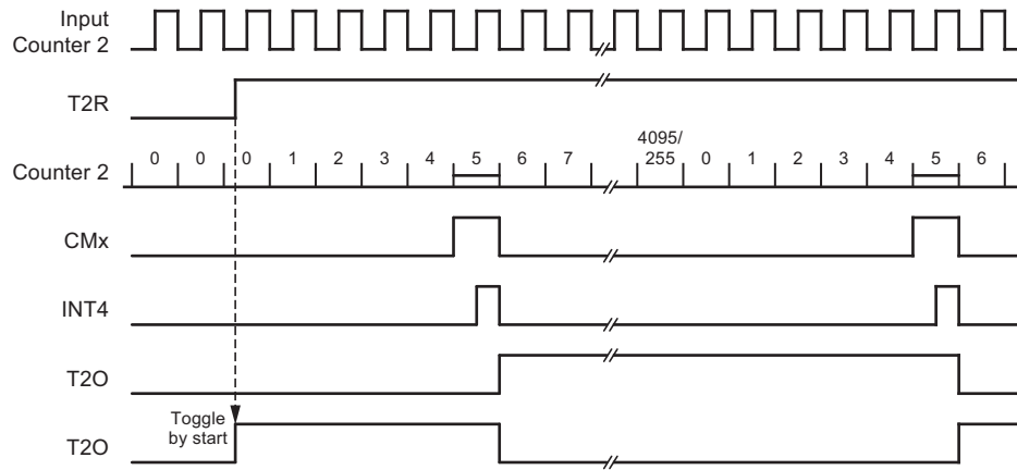
Figure 4-15. Pulse Generator — Timer Output Toggles with Timer Start If T2TS-Bit is Set
