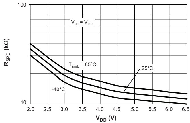
Figure 7-15. Strong Pull-down Resistor versus V_{DD}
