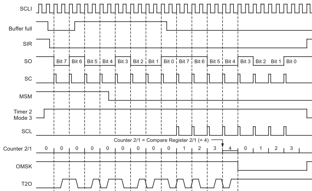
Figure 4-36. Manchester Modulation 2
