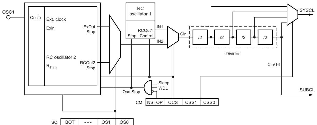
Figure 3-12. Clock Module
