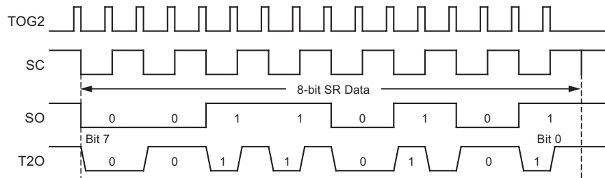
Figure 4-34. Bi-phase Modulation 1
