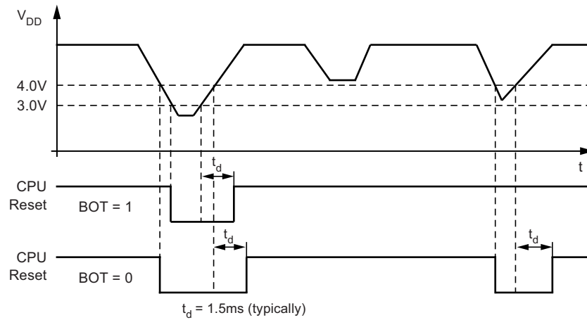
Figure 3-8. Brown-out Detection
