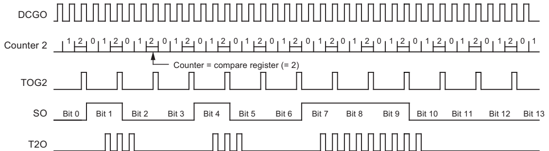
Figure 4-33. Carrier Frequency Burst Modulation with the SSI Internal Data Output
