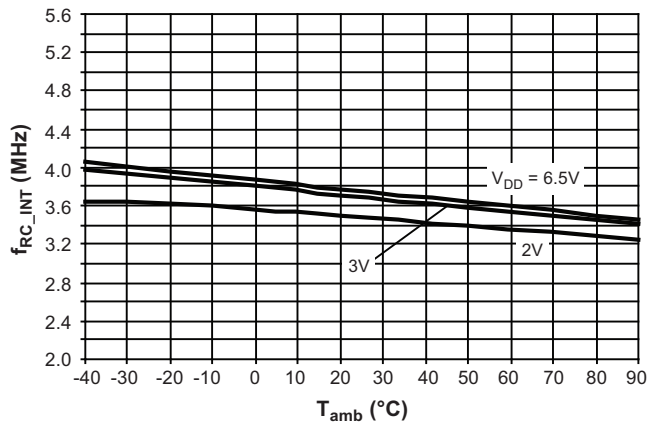
Figure 7-8. Internal RC Frequency versus T_{amb}
