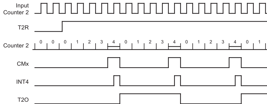
Figure 4-14. Interrupt Timer/Square Wave Generator — Output Toggles with Each Edge Compare Match Event
