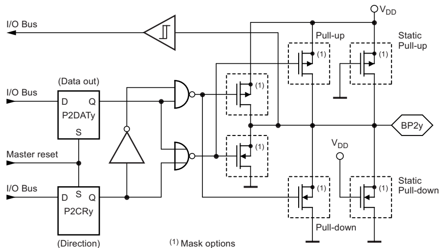
Figure 4-2. Bi-directional Port 2
