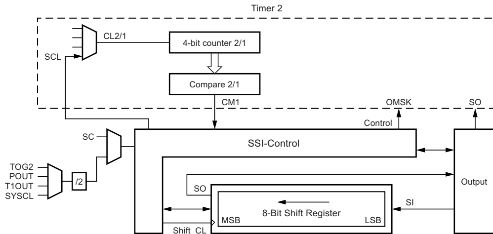
Figure 4-31. SSI Output Masking Function
