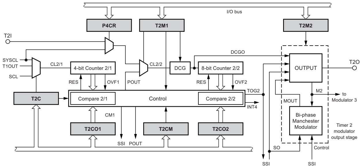
Figure 4-9. Timer 2
