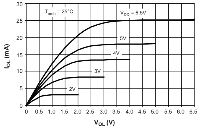
Figure 7-16. Output Low Current versus Output Low Voltage
