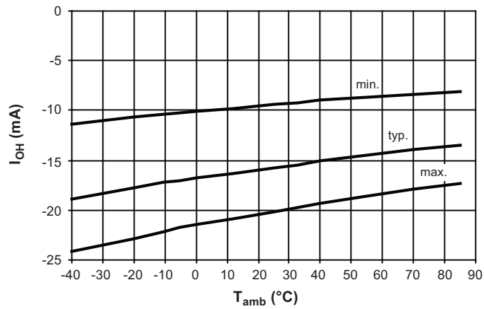
Figure 7-17. Output High Current versus T_{amb} = 25^\circ\text{C} , V_{DD} = 6.5\text{V} , V_{OH} = 0.8 \times V_{DD}
