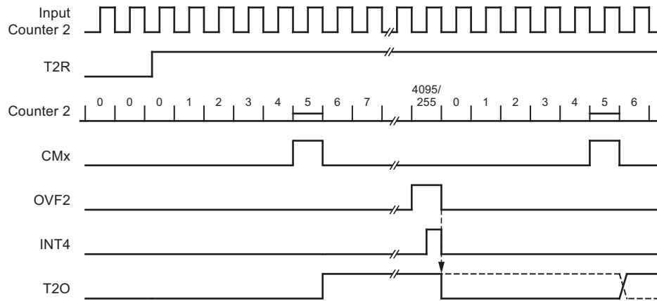
Figure 4-16. Pulse Generator — Timer Toggles with Timer Overflow and Compare Match
