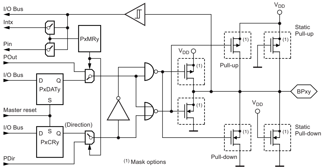
Figure 4-5. Bi-directional Port 4
