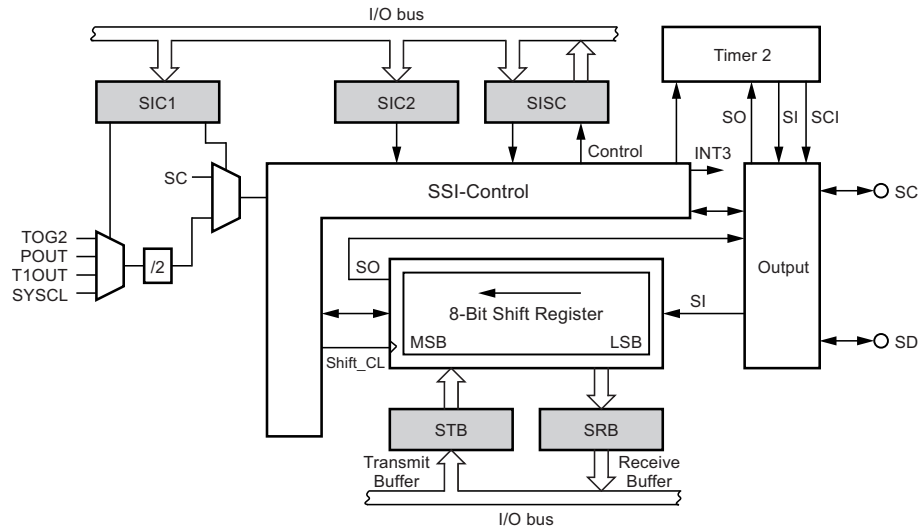
Figure 4-23. Block Diagram of the Synchronous Serial Interface
