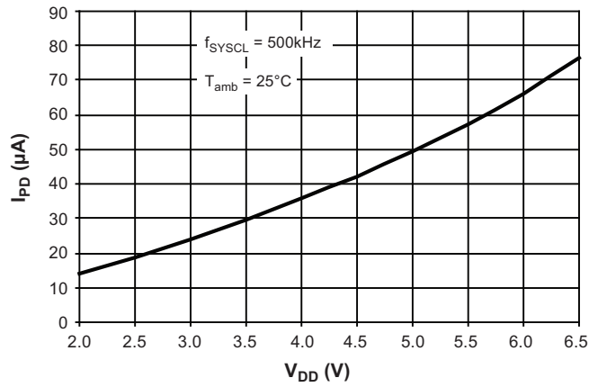
Figure 7-4. Power-down Supply Current versus V_{DD}
