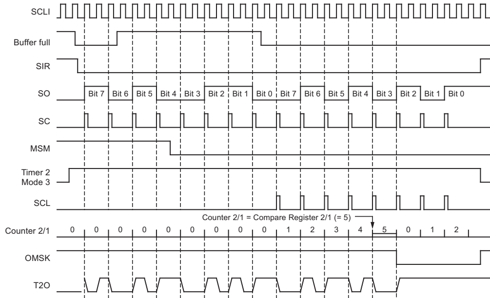
Figure 4-37. Bi-phase Modulation 2
