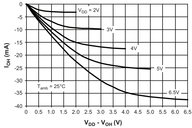
Figure 7-13. Output High Current versus V_{DD} - Output High Voltage
