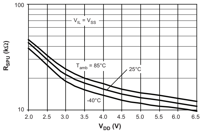
Figure 7-12. Strong Pull-up Resistor versus V_{DD}
