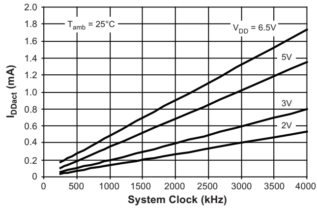
Figure 7-1. Active Supply Current versus Frequency
