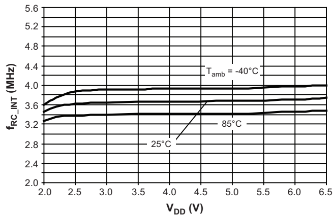
Figure 7-5. Internal RC Frequency versus V_{DD}
