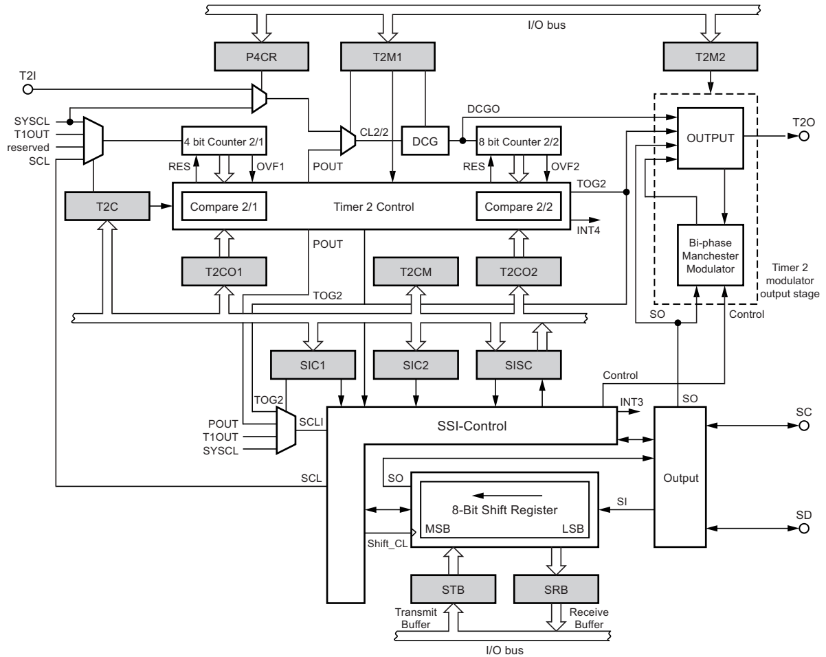
Figure 4-32. Combination Timer 2 and SSI
