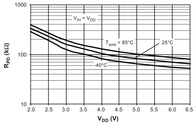
Figure 7-14. Pull-down Resistor versus V_{DD}
