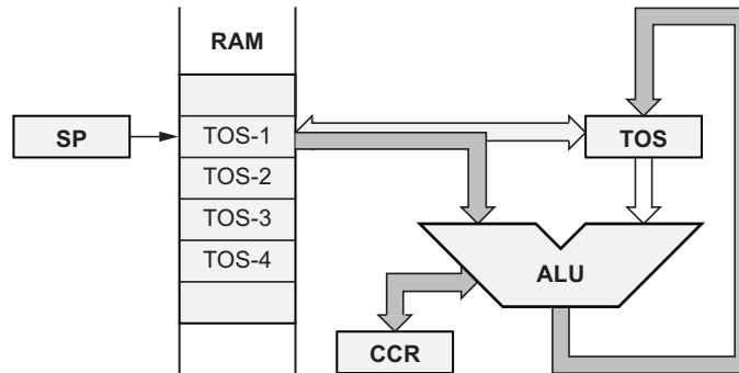
Figure 3-5. ALU Zero-address Operations
