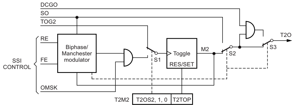
Figure 4-13. Timer 2 Modulator Output Stage
