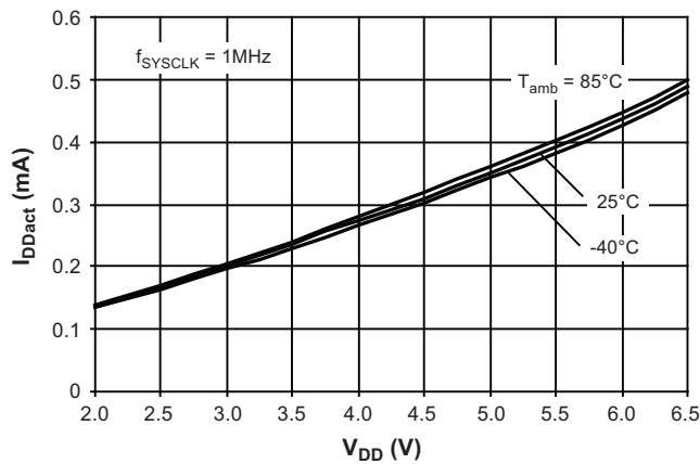
Figure 7-3. Active Supply Current versus V_{DD}
