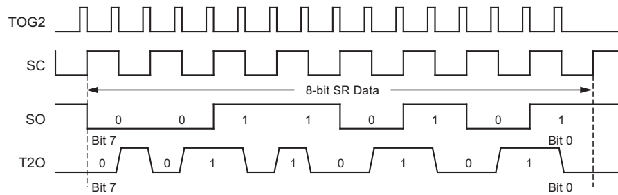
Figure 4-20. Manchester Modulation
