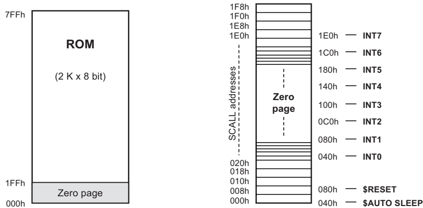
Figure 3-2. ROM Map of ATA6020N
