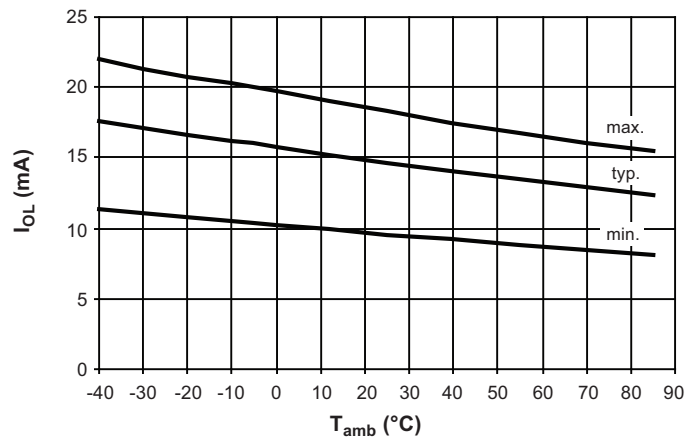
Figure 7-18. Output Low Current versus T_{amb} , V_{DD} = 6.5\text{V} , V_{OL} = 0.2 \times V_{DD}
