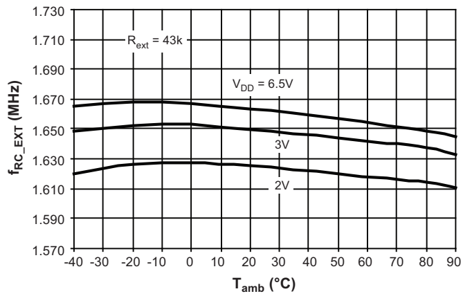
Figure 7-9. External RC Frequency versus T_{amb}
