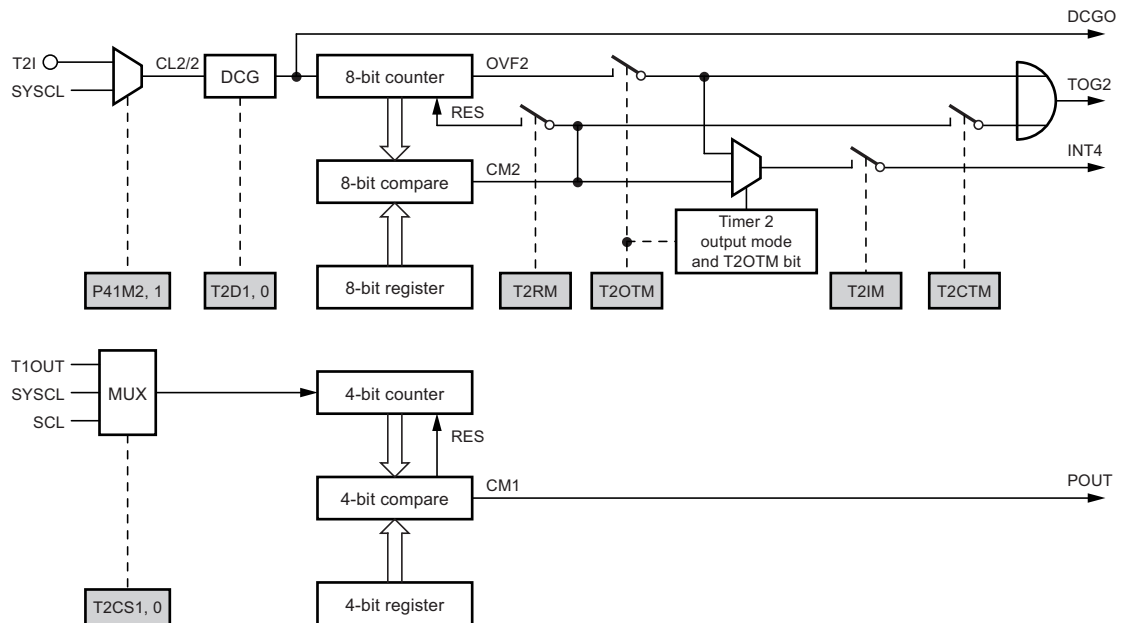
Figure 4-12. 4-/8-bit Compare Counter
