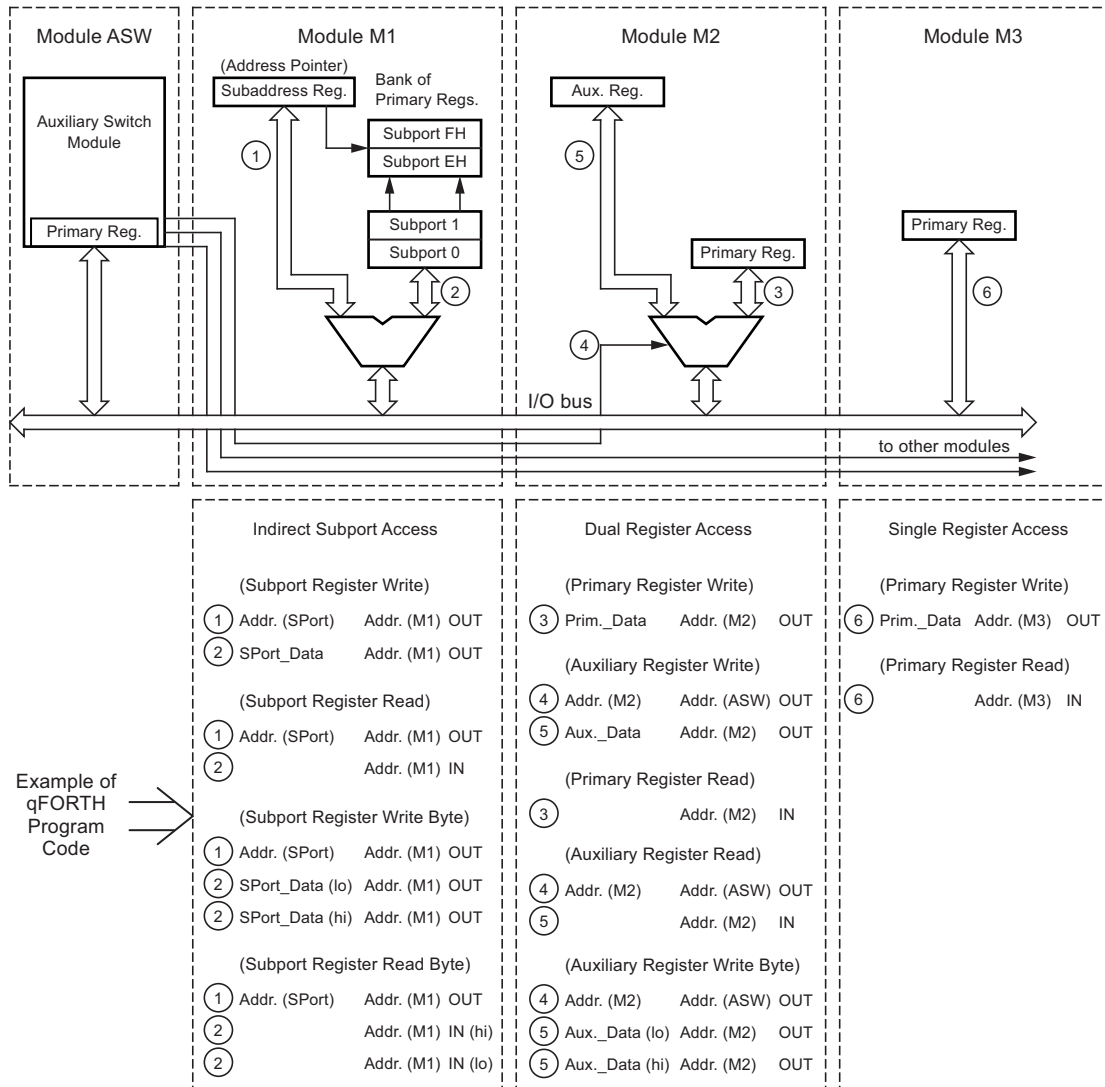
Figure 4-1. Example of I/O Addressing
