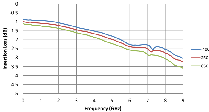
Figure 19. Insertion Loss vs. Temperature
