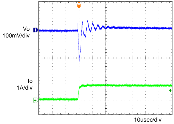
Figure 4. Transient Response (0→1.0A) Co=1μF, Ta=25°C
