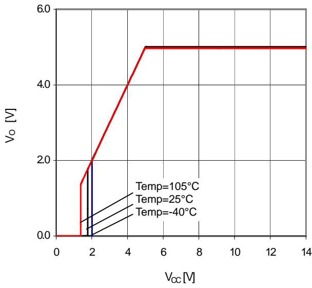
Figure 27. V_{CC}-V_o ( I_o=0mA )
