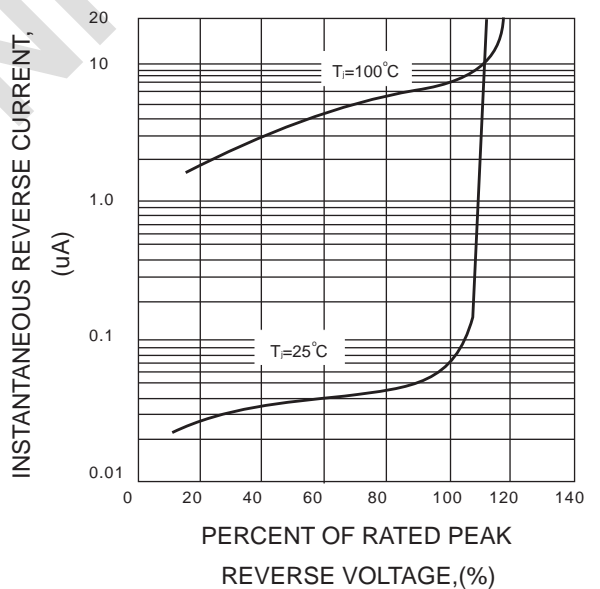
FIG.4-TYPICAL REVERSE CHARACTERISTICS
