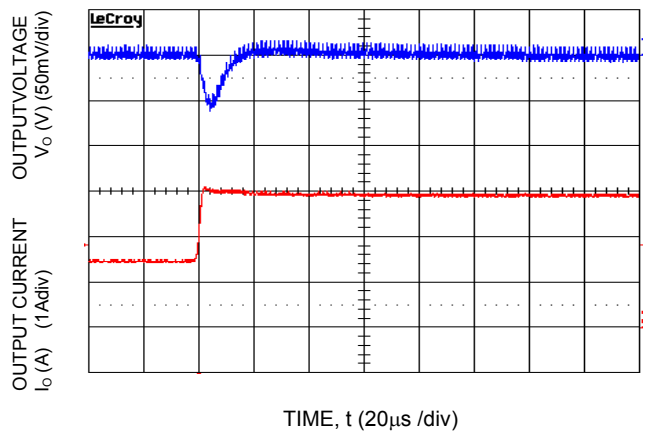
Figure 28. Transient Response to Dynamic Load Change from 50% to 100% at 12Vin, C_{out}=2x47\mu\text{F} , C_{Tune}=2200\text{pF} & R_{Tune}=261
