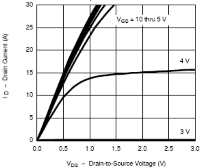
Output Characteristics
