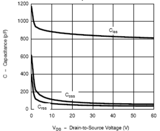
Capacitance
