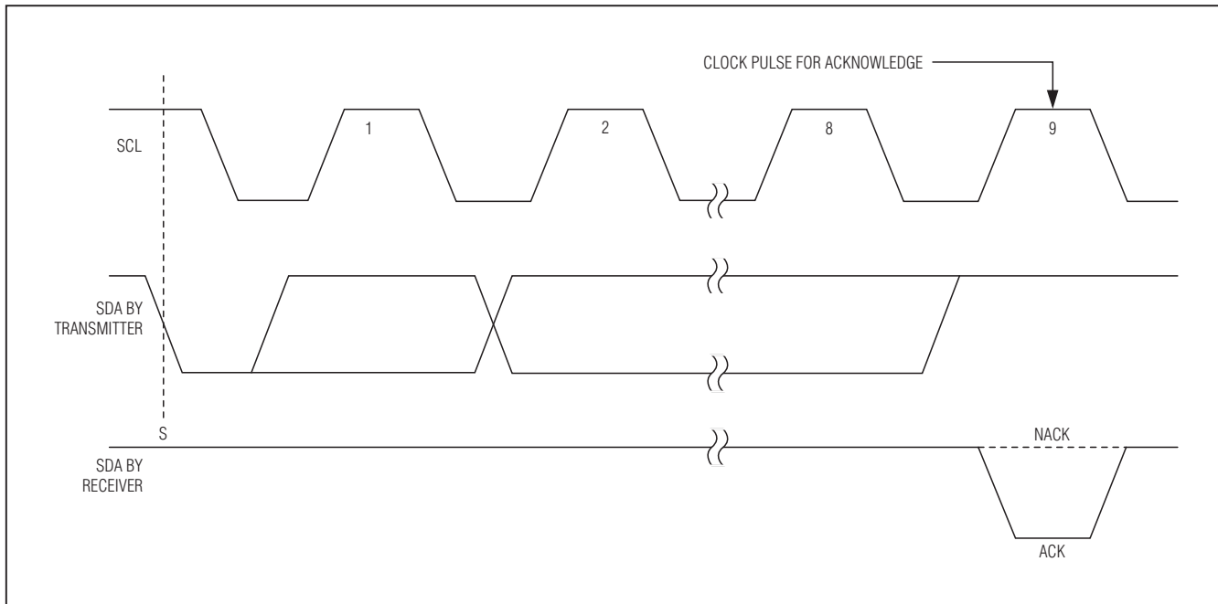
Figure 10. Acknowledge
