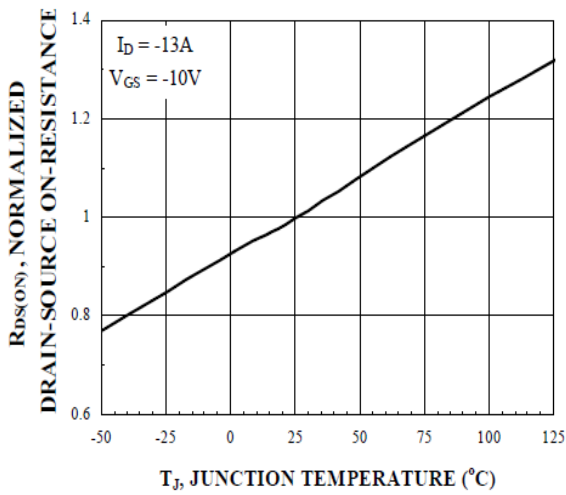
Figure 3. On-Resistance Variation with Temperature
