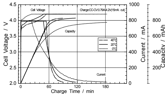
Charge characteristics
