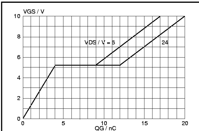
Fig. 13. Typical turn-on gate-charge characteristics. V_{GS} = f(Q_G) ; conditions: I_D = 40 A; parameter V_{DS}
