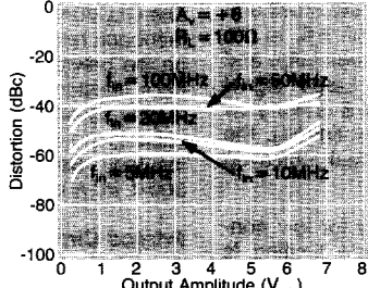
2nd Harmonic Distortion, C L = 25pF
