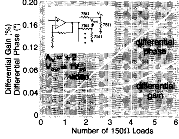
Differential Gain and Phase vs Load
