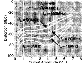
3rd Harmonic Distortion, C L = 25pF
