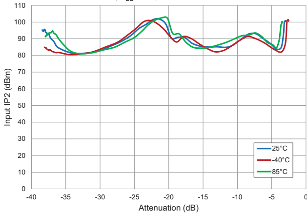
Input IP2 versus Attenuation RF 2GHz, V_{DD}=3.3V , P_{in}=+20dBm/Tone
