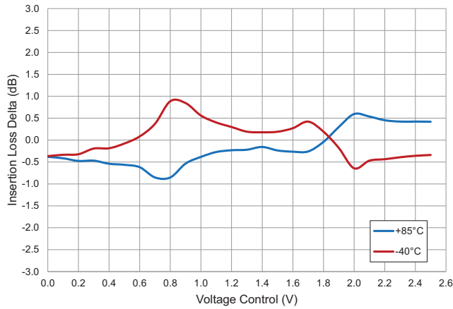
Insertion Loss Relative to +25°C
