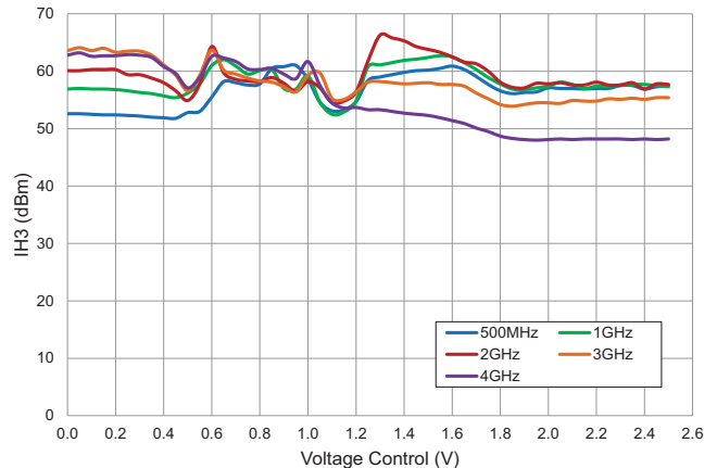
3rd Harmonic IH3 versus Voltage Control V_{DD}=3.3V , P_{in}=+20dBm , Temp=+25^{\circ}C
