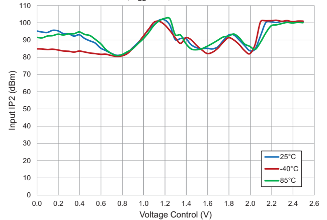
Input IP2 versus Voltage Control RF 2GHz, V_{DD}=3.3V , P_{in}=+20dBm/Tone
