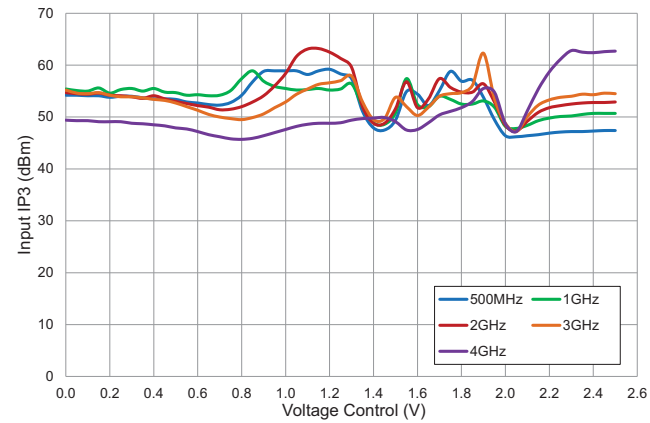
Input IP3 versus Voltage Control V_{DD}=3.3V , P_{in}=+20dBm/Tone , Temp= +25^{\circ}C
